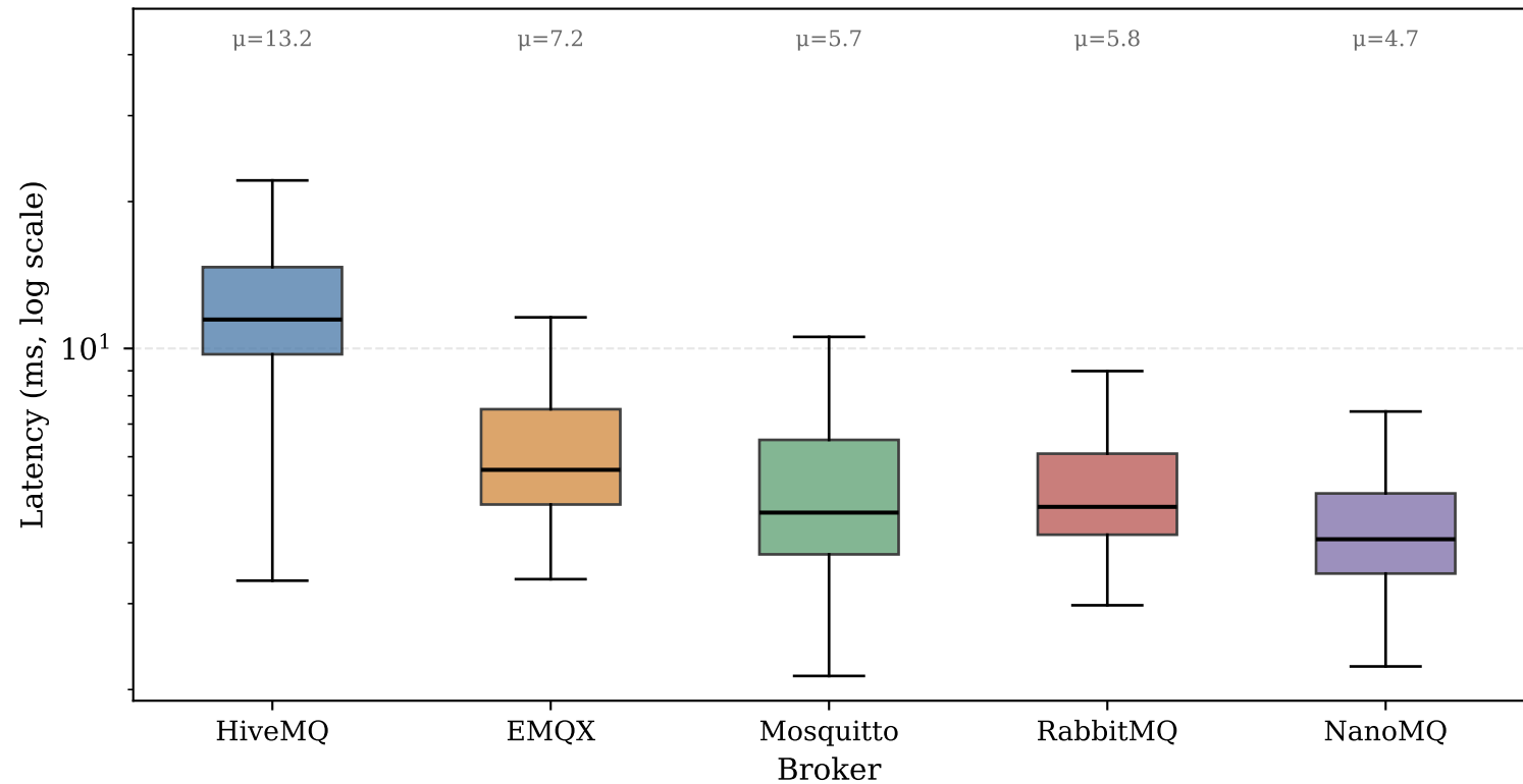
End-to-End Latency — 1 KB Payload (QoS 0)
