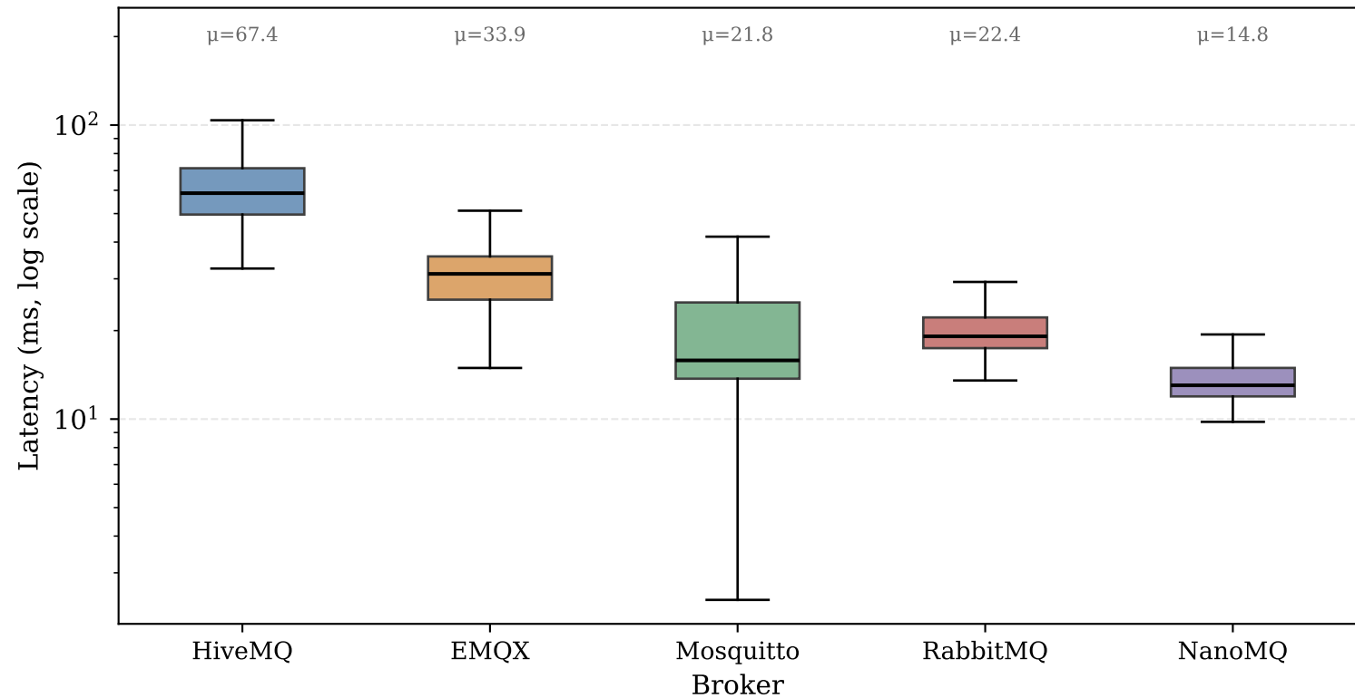
End-to-End Latency — 1 MB Payload (QoS 0)
