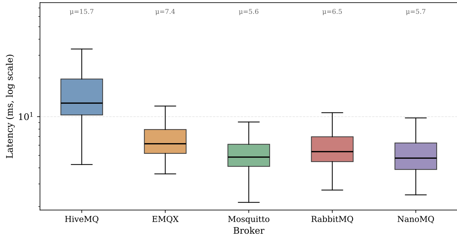
End-to-End Latency — 35 KB Payload (QoS 0)
