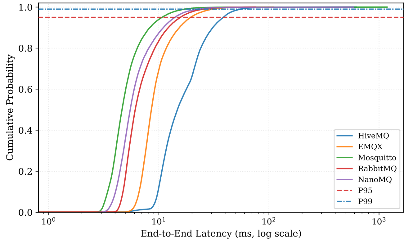
Latency CDF — 125 KB Payload (QoS 0)
