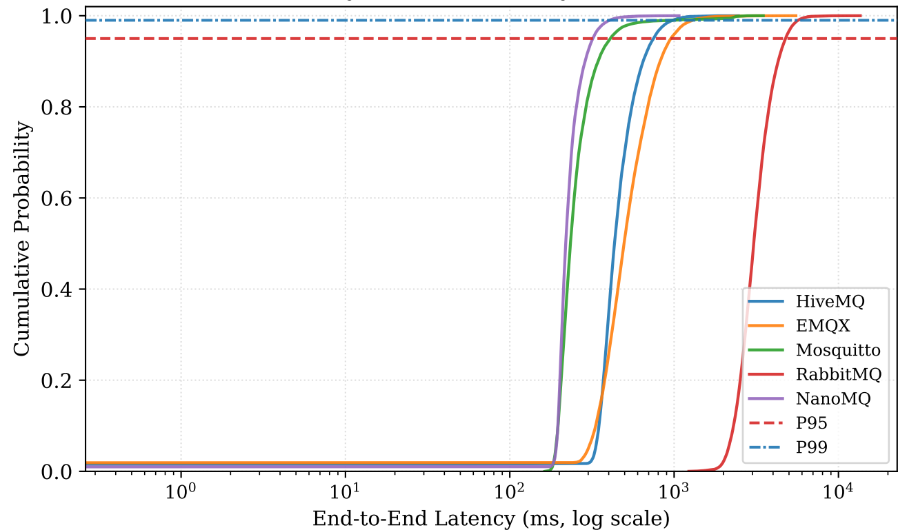
Latency CDF — 16 MB Payload (QoS 0)
