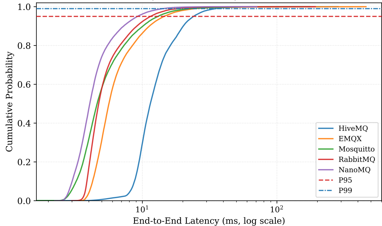
Latency CDF — 1 KB Payload (QoS 0)
