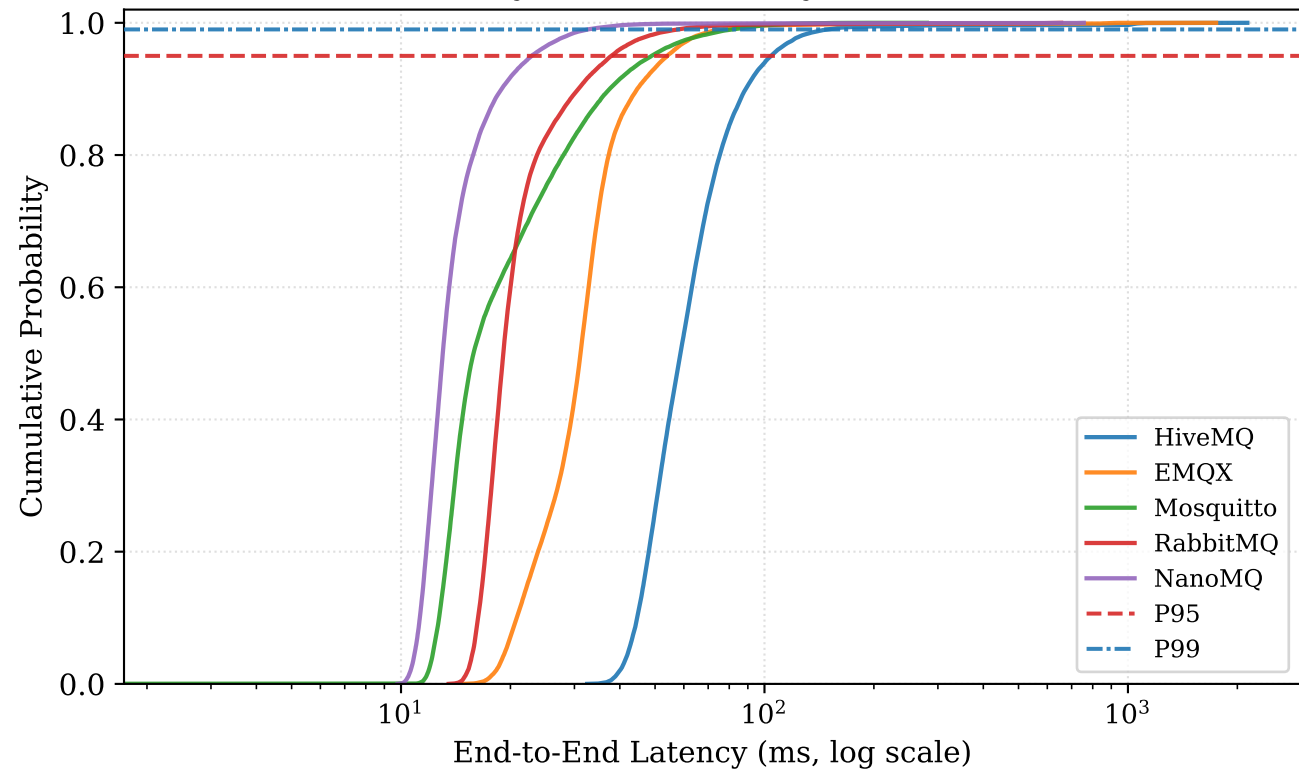
Latency CDF — 1 MB Payload (QoS 0)
