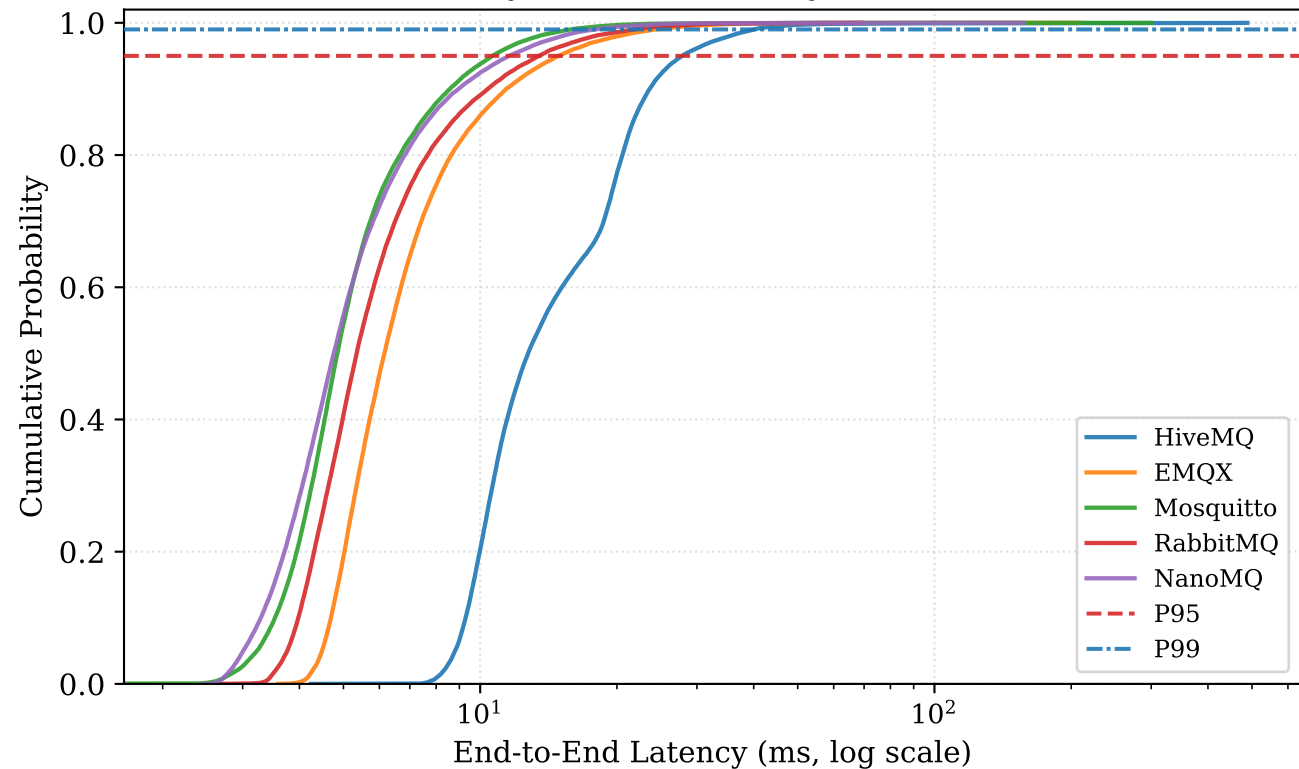
Latency CDF — 35 KB Payload (QoS 0)
