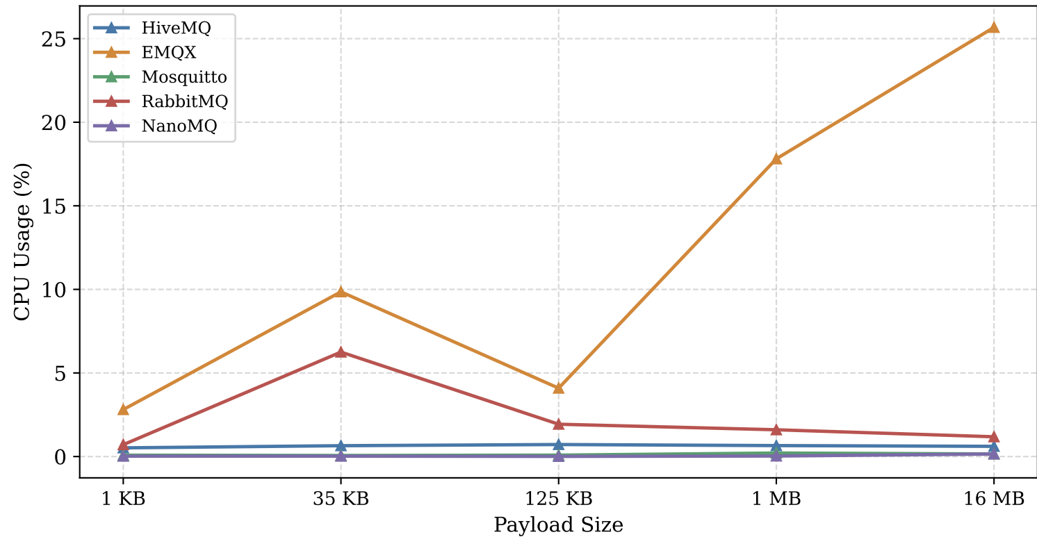
Average Broker CPU Usage vs. Payload Size (QoS 0)
