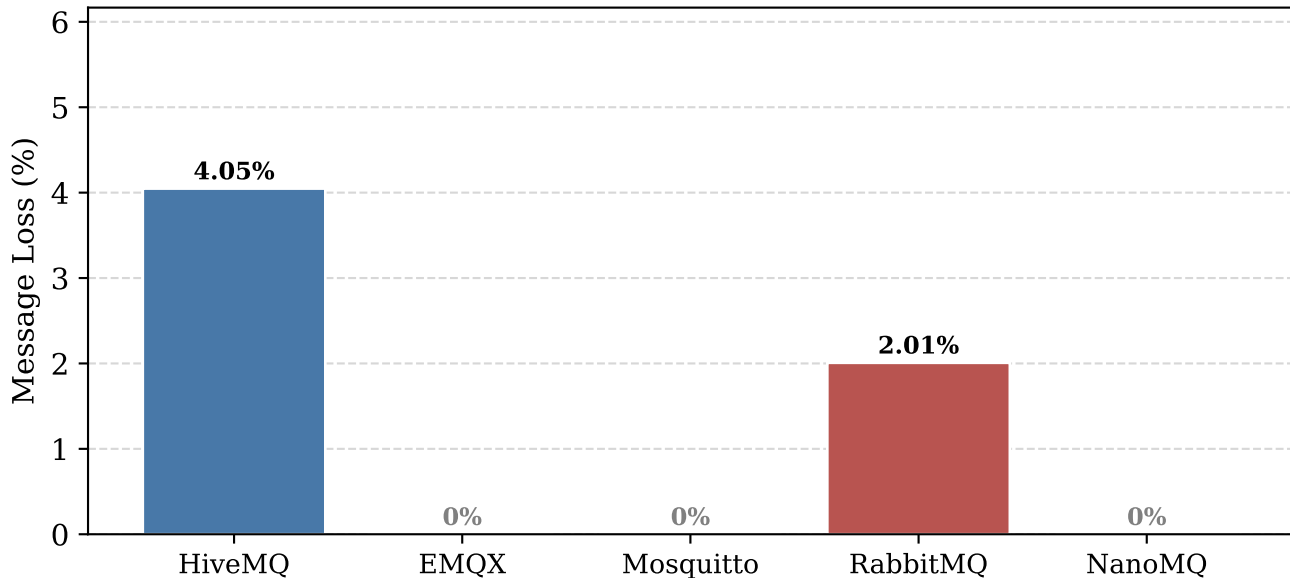
Message Loss Rate — 16 MB Payload (QoS 0)
