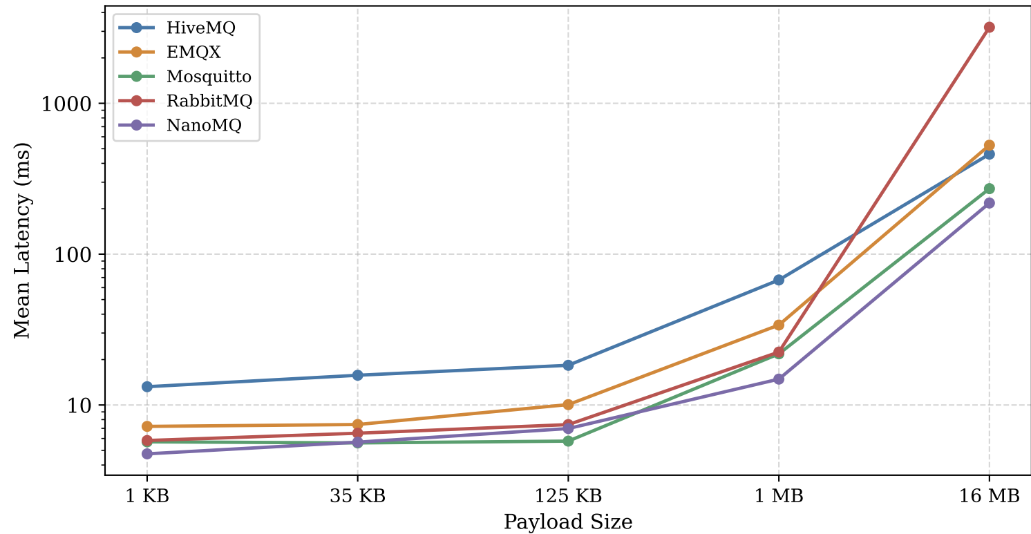
Mean End-to-End Latency vs. Payload Size (QoS 0)
