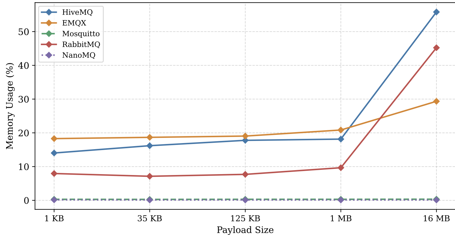
Average Broker Memory Usage vs. Payload Size (QoS 0)
