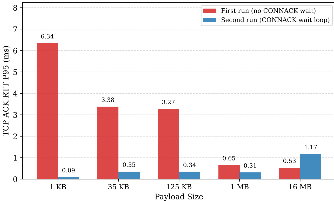
HiveMQ — RTT P95 Before and After CONNACK Wait-Loop Fix (QoS 0)
