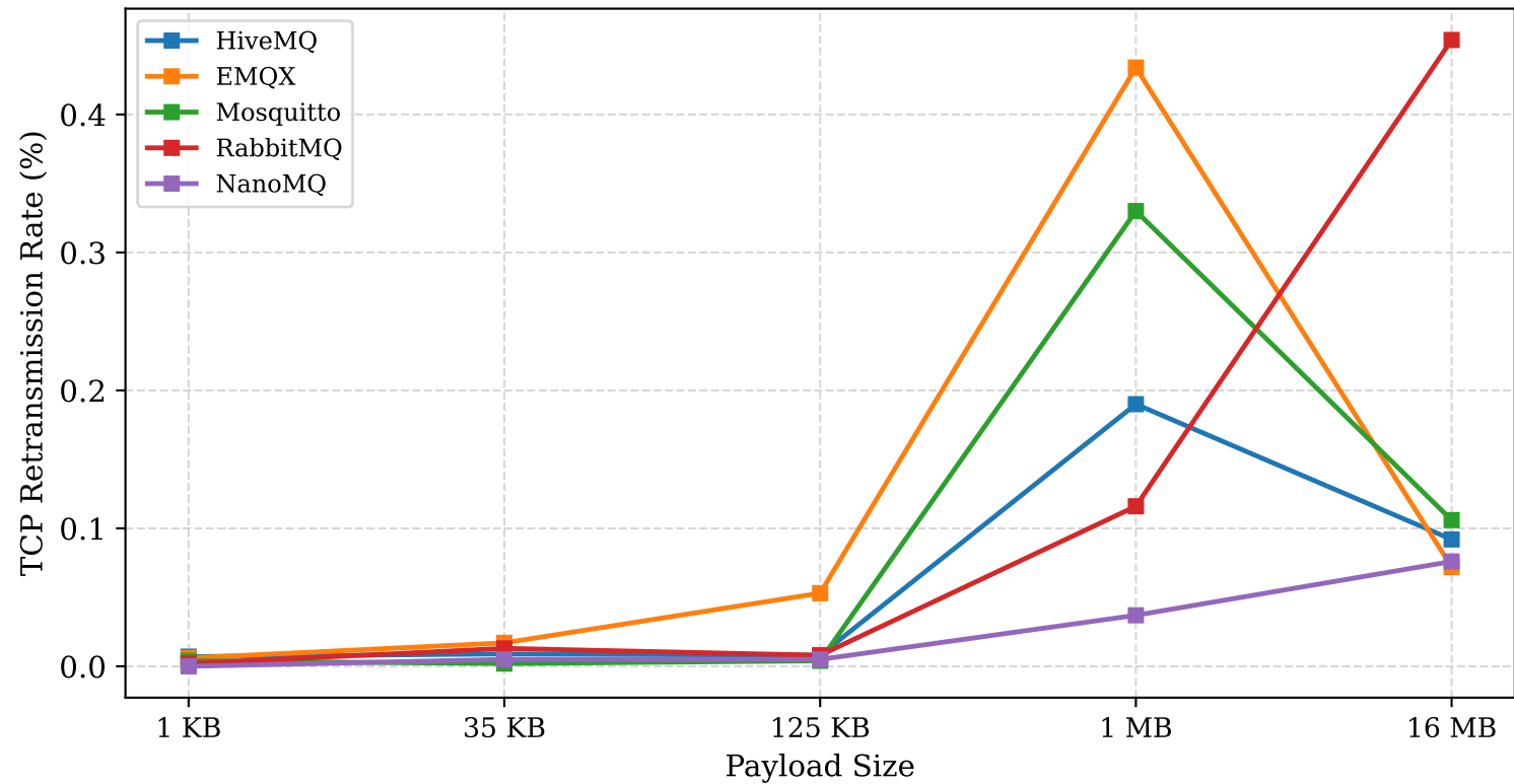
TCP Retransmission Rate vs. Payload Size (QoS 0)
