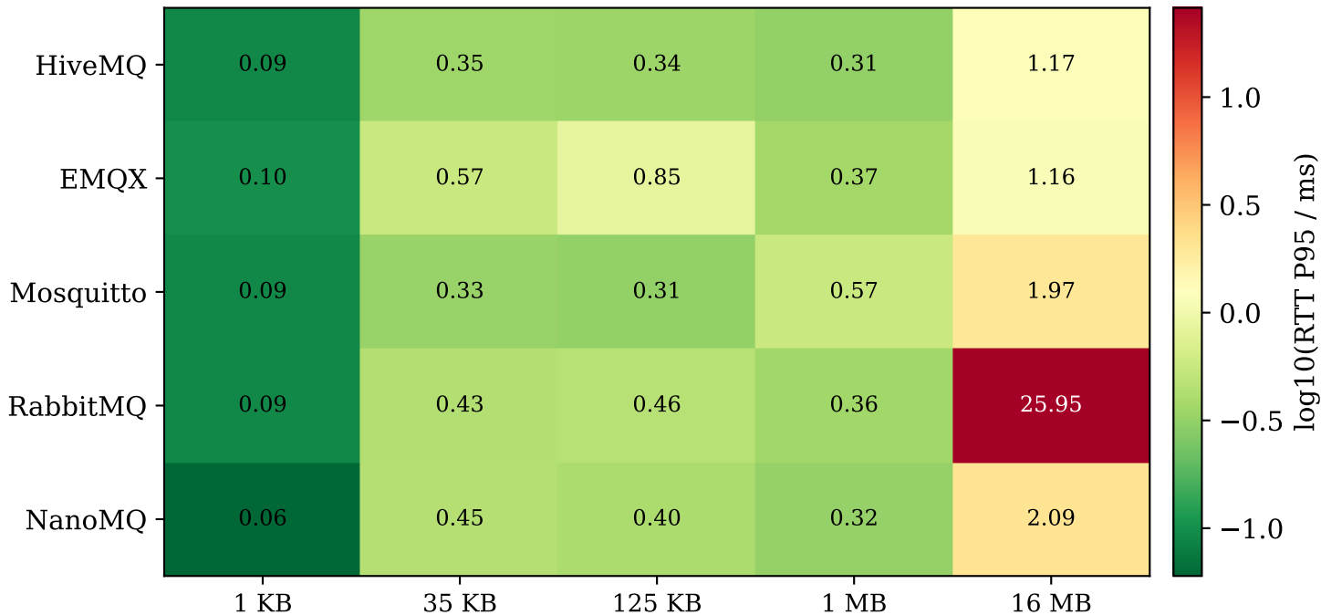
TCP RTT P95 Heatmap — \log_{10}(\text{ms}) (QoS 0)
