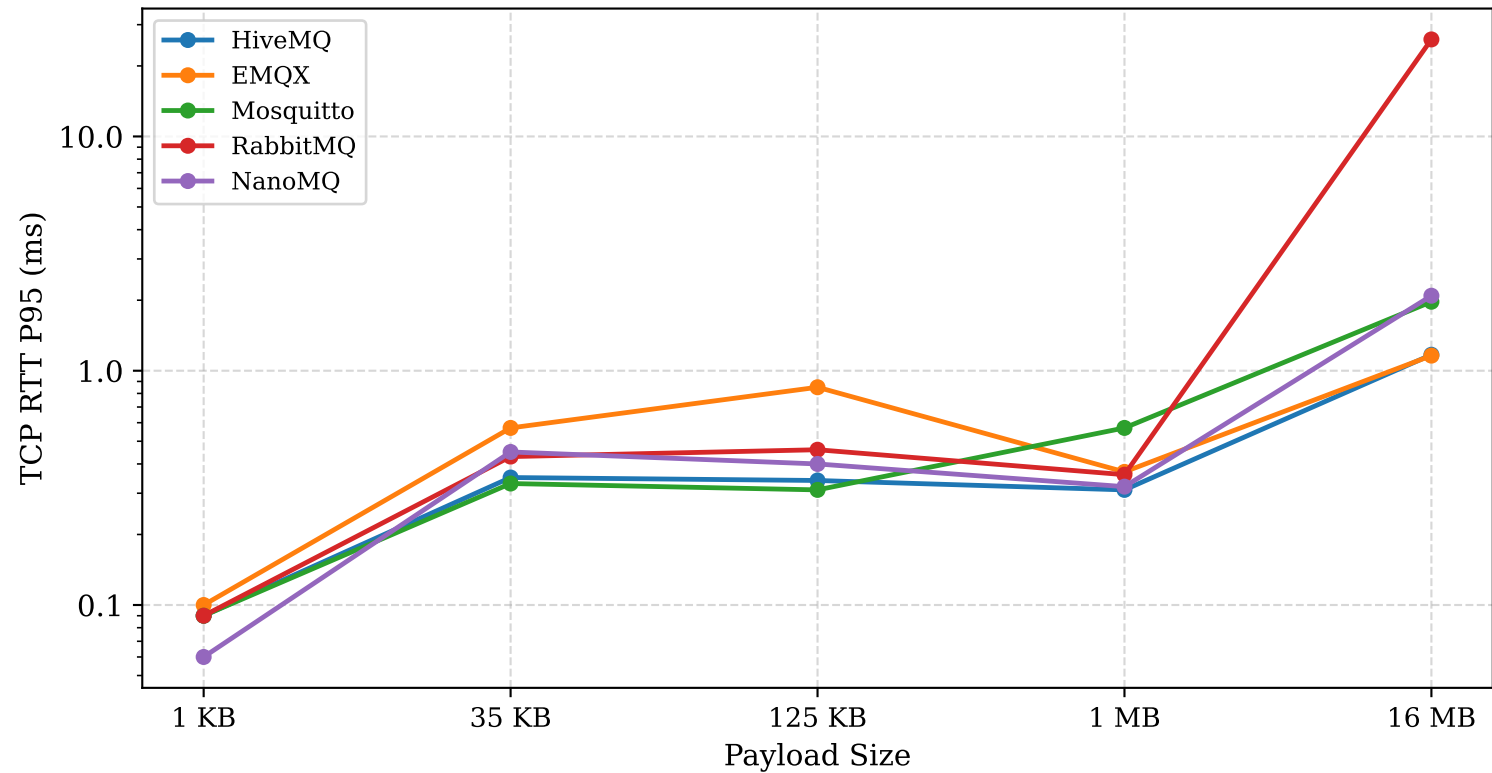
TCP 95th-Percentile Round-Trip Time vs. Payload Size (QoS 0)
