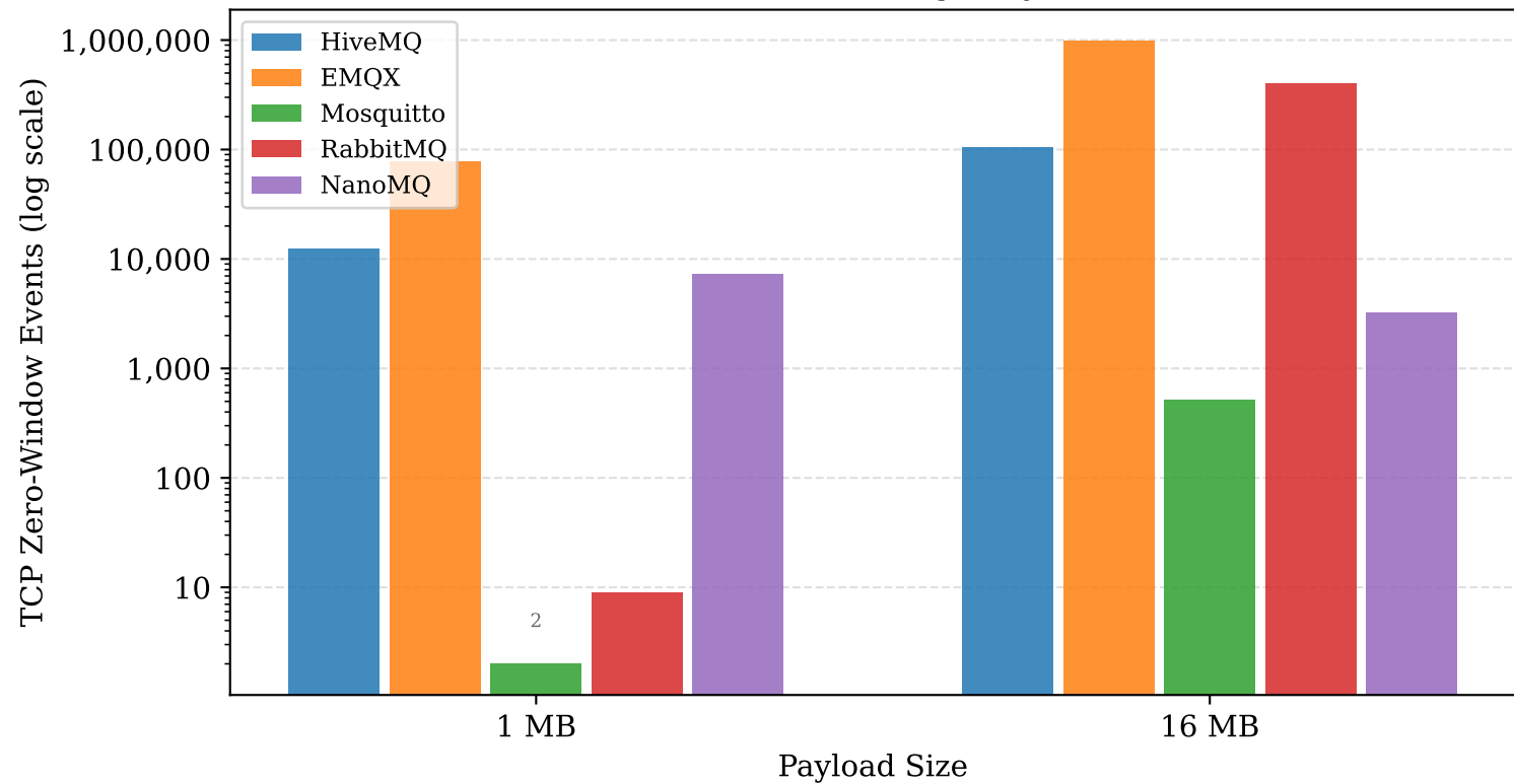
TCP Zero-Window Events at Large Payload Sizes (QoS 0)
