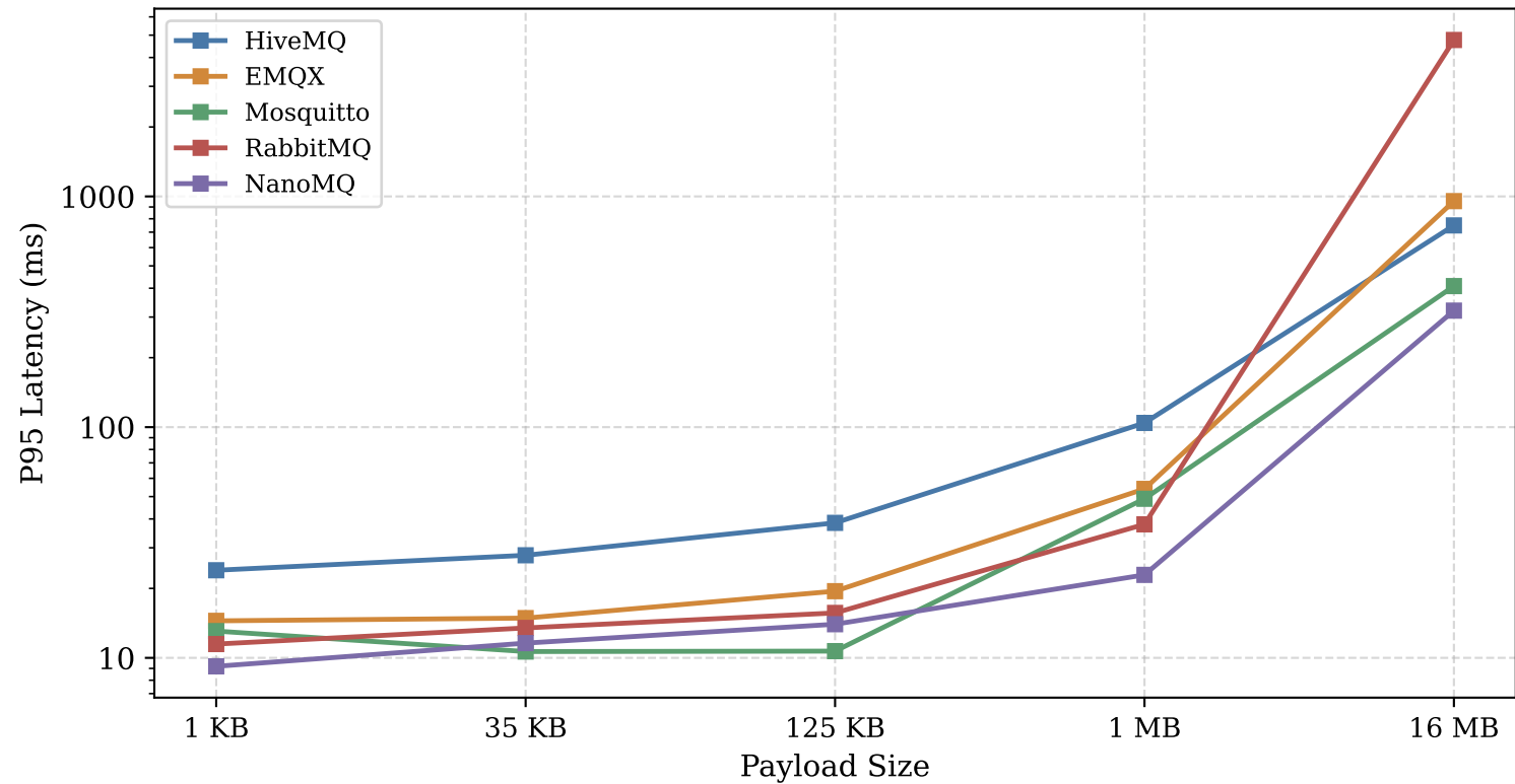
95th-Percentile Latency vs. Payload Size (QoS 0)
