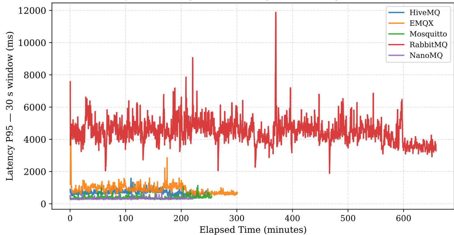
Temporal Stability of P95 Latency — 16 MB Payload (QoS 0)
