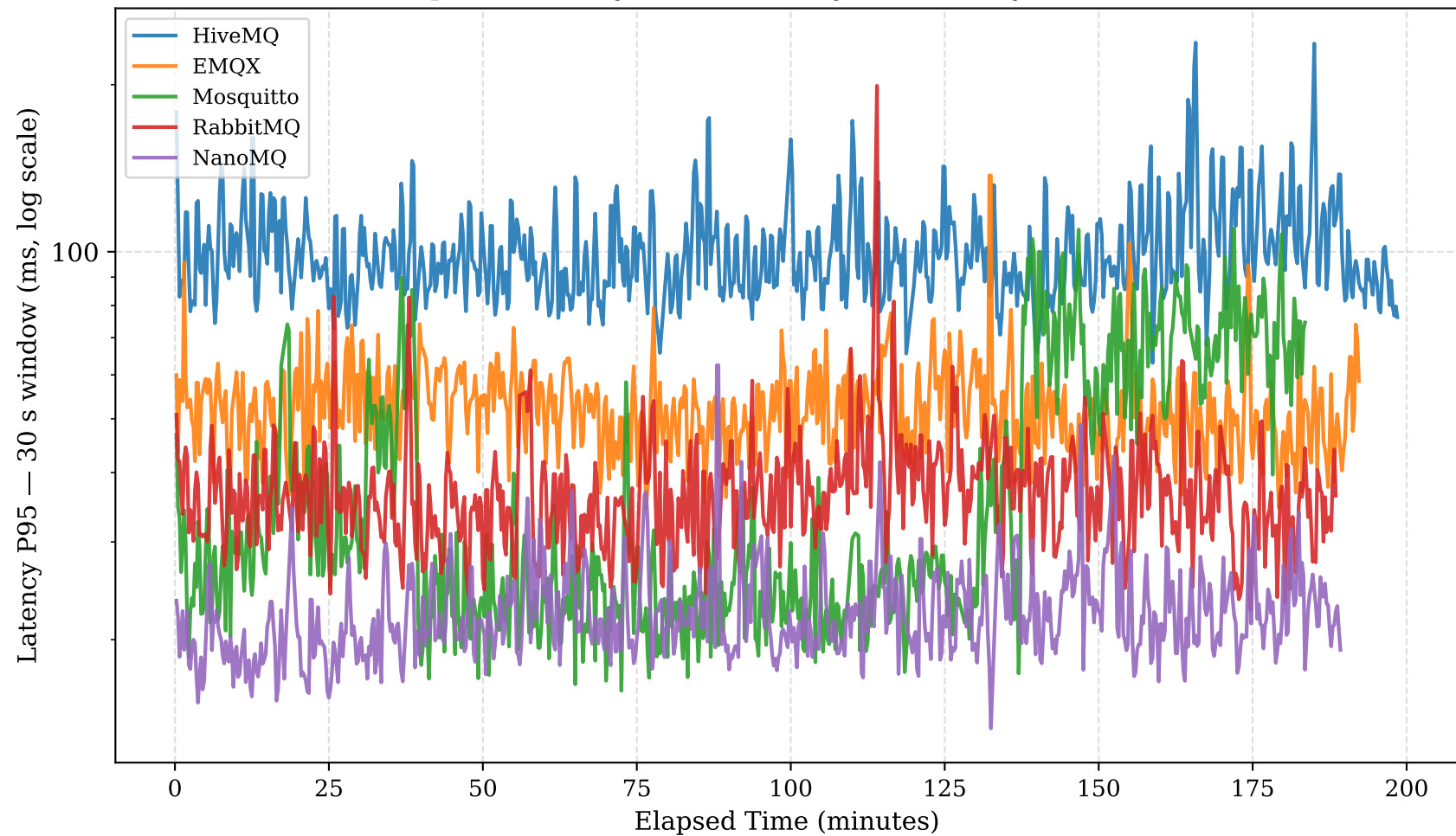
Temporal Stability of P95 Latency — 1 MB Payload (QoS 0)
