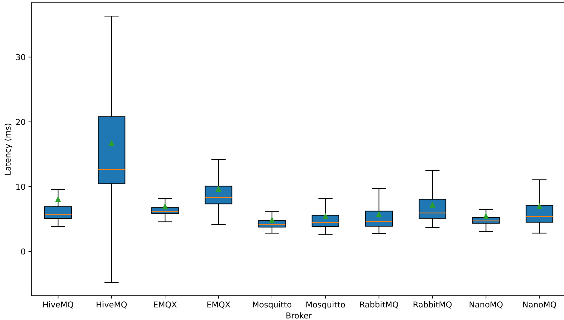
Latency — GATEWAY1 — QOS0 — 128 KB Payload
