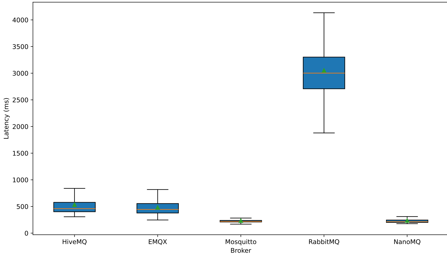
Latency — GATEWAY1 — QOS0 — 16 MB Payload
