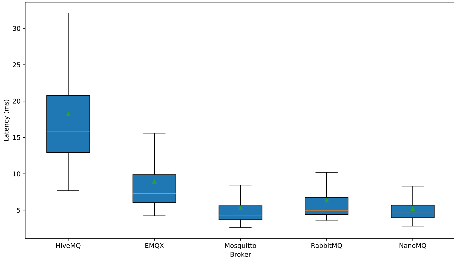
Latency — GATEWAY1 — QOS0 — 35 KB Payload
