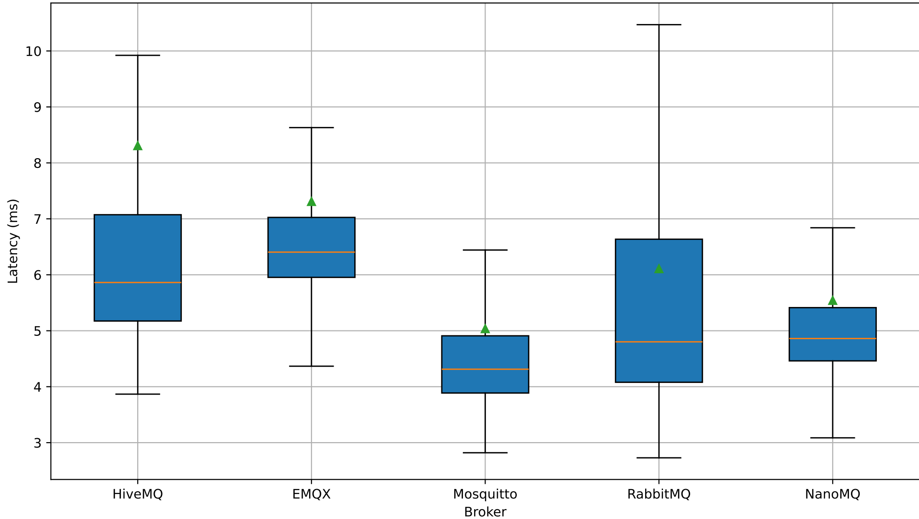
Latency — 128 KB Payload
