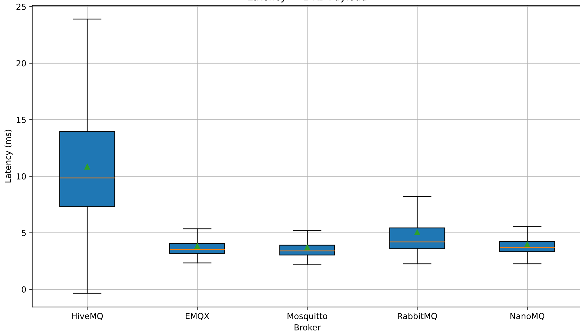
Latency — 1 KB Payload
