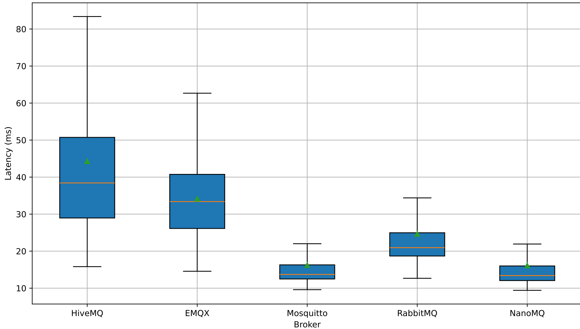
Latency — 1 MB Payload
