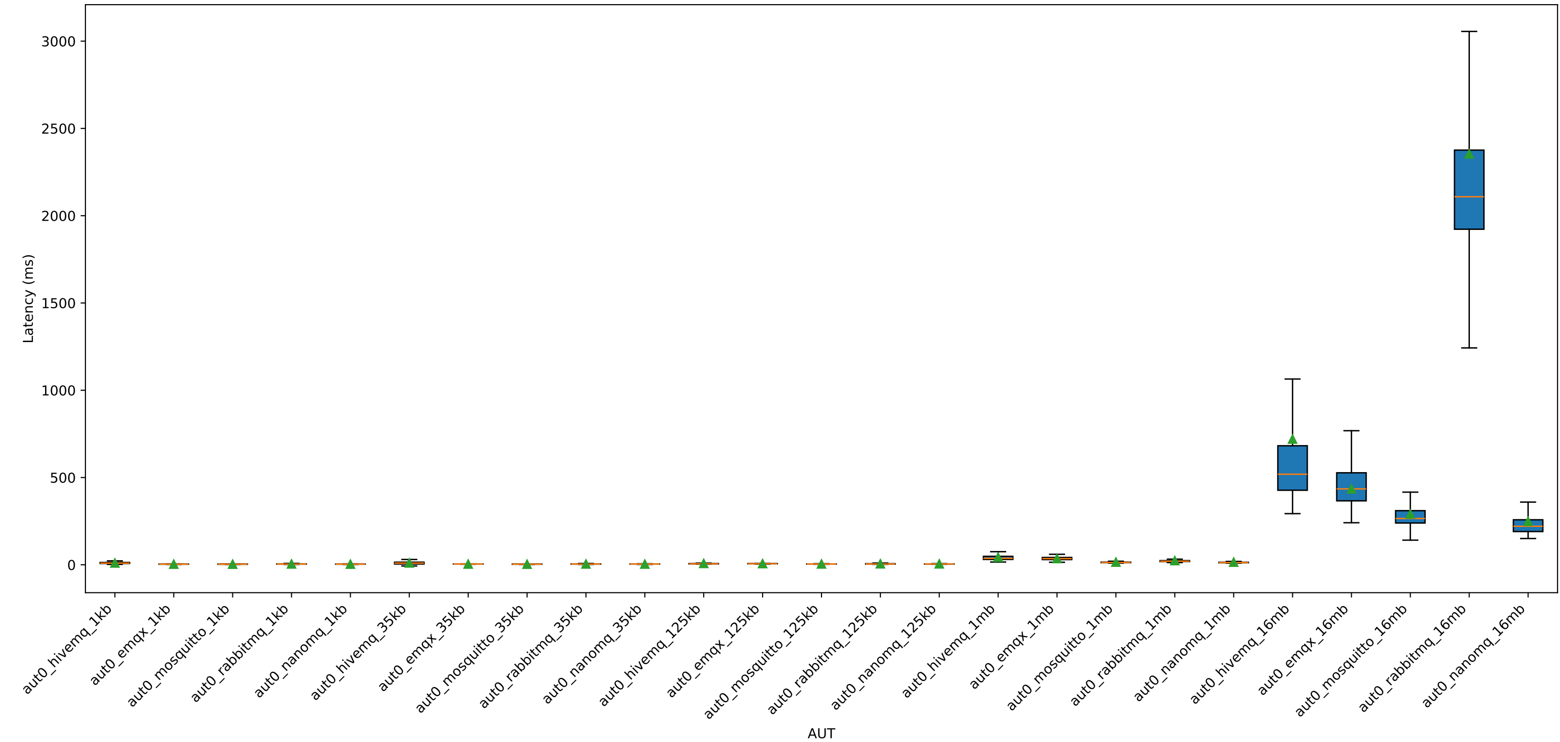
Latency for GATEWAY1: QOS0
