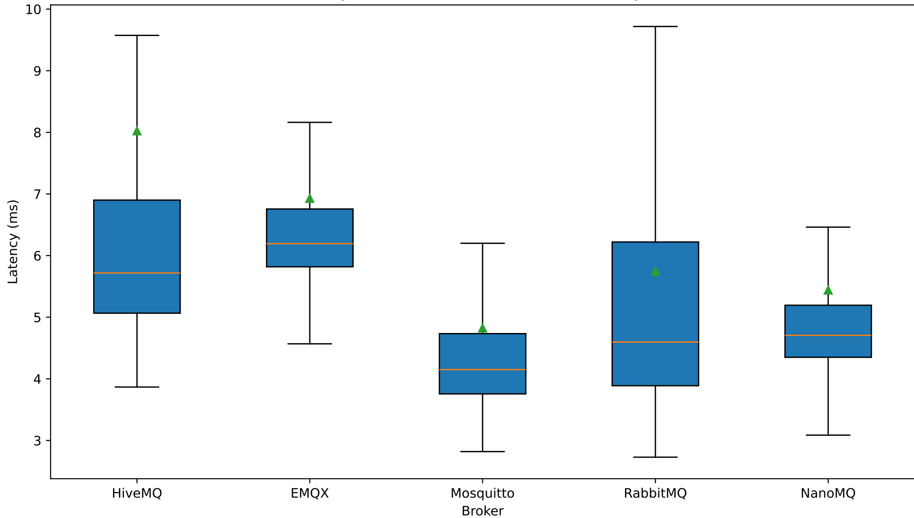
Latency — GATEWAY1 — QOSO — 128 KB Payload
