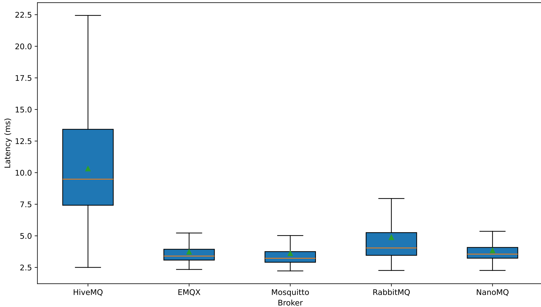
Latency — GATEWAY1 — QOS0 — 1 KB Payload
