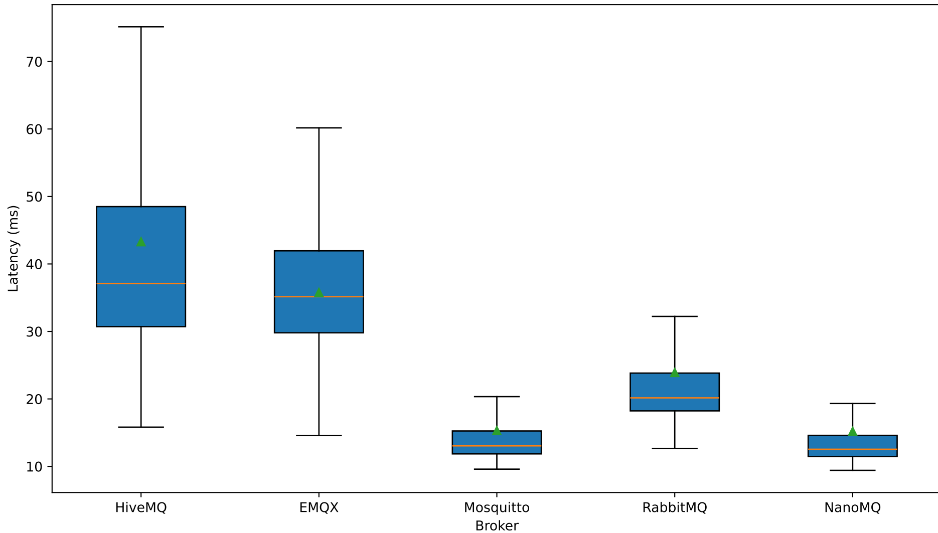
Latency — GATEWAY1 — QOS0 — 1 MB Payload
