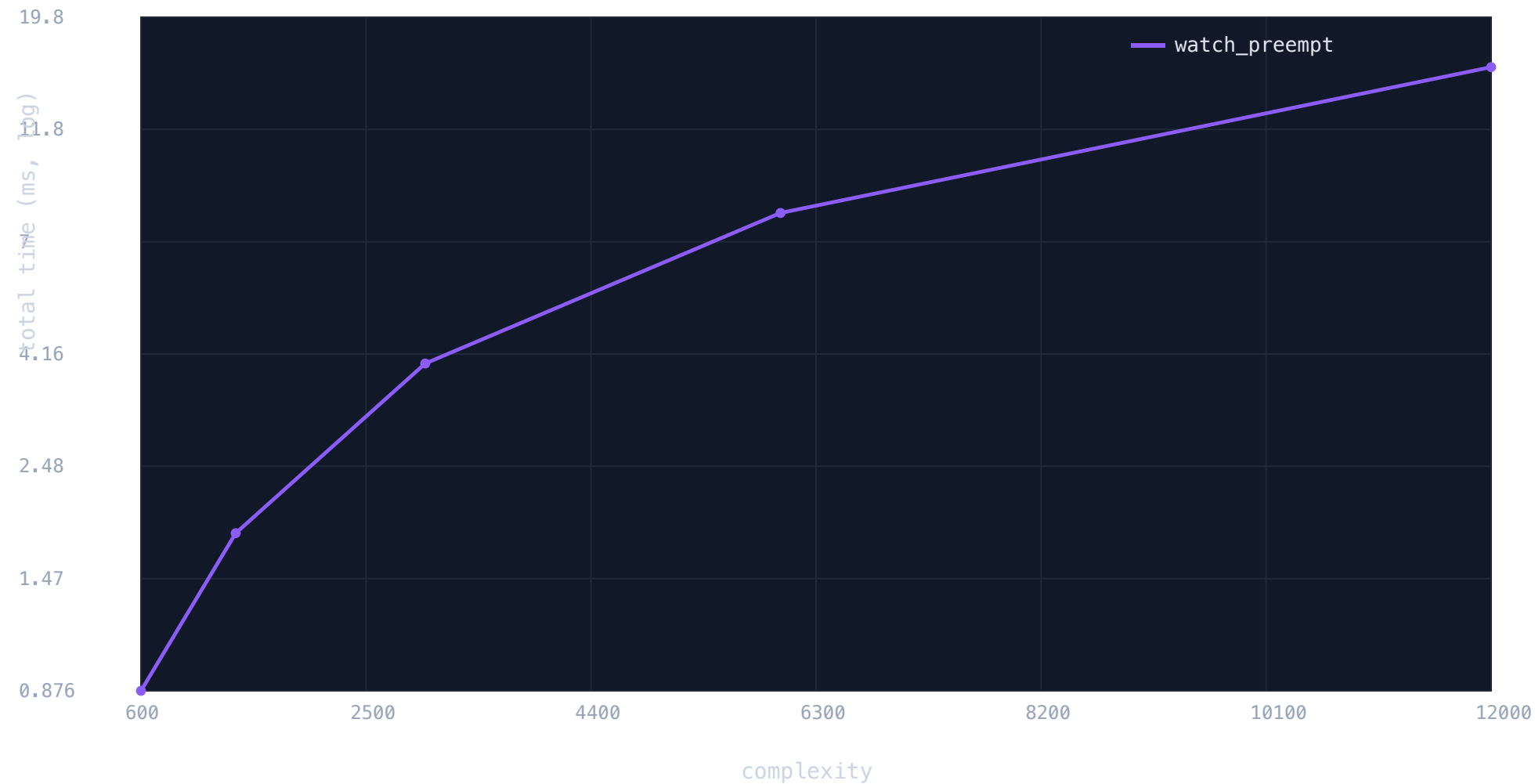
watch preemption cost – total time vs complexity (log Y)
