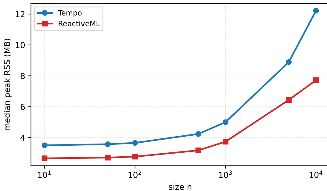
B5 Nested preemption
