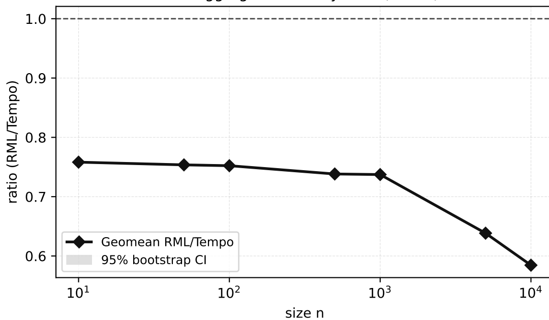
B6 Aggregate memory ratio (B1-B5)
