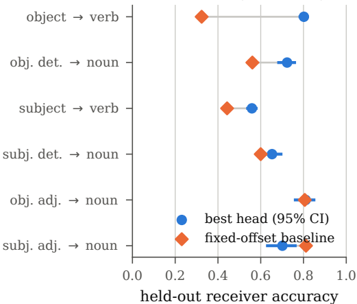
DiffuGPT-S (144 heads)
