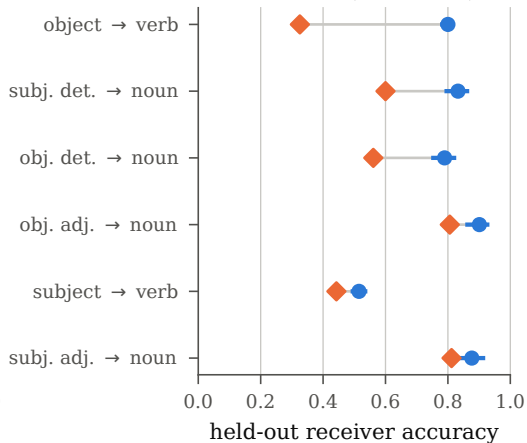
Dream-7B (784 heads)
