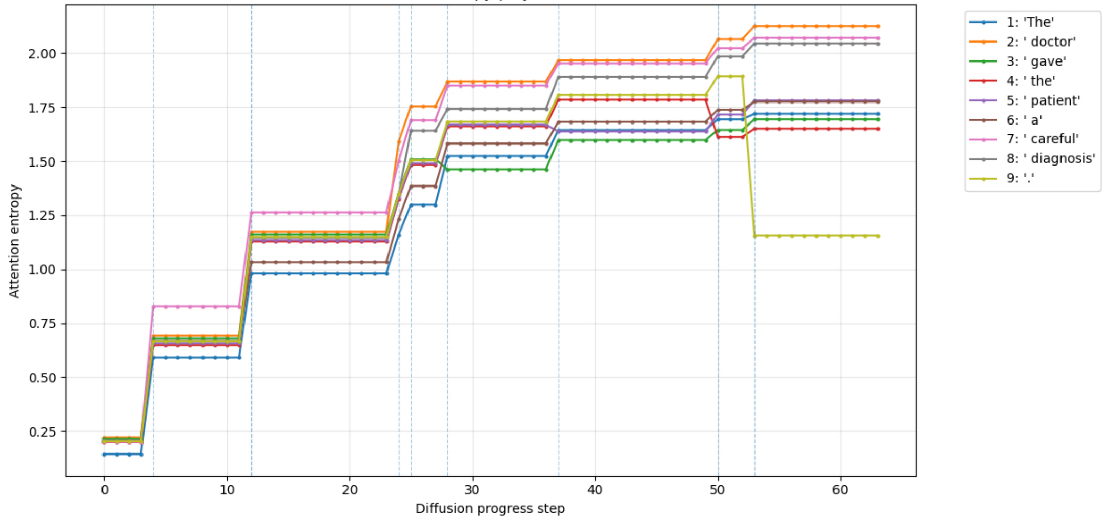
DiffuGPT attention entropy | layer 0, head 0, seed 42
