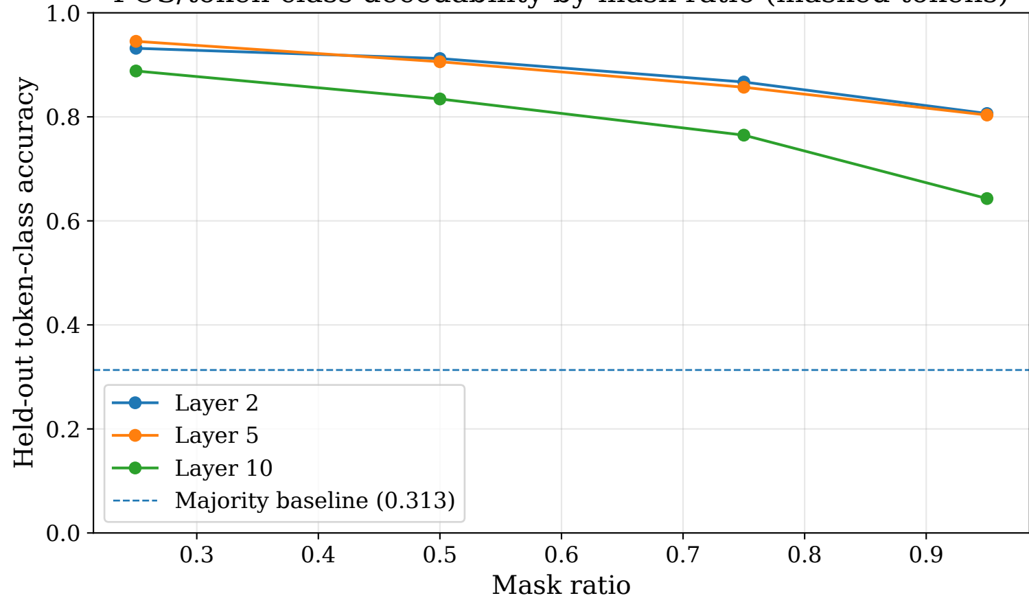
POS/token-class decodability by mask ratio (masked tokens)
