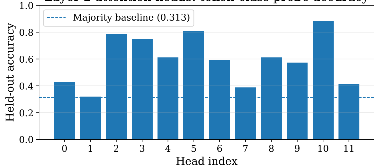
Layer 2 attention heads: token-class probe accuracy
