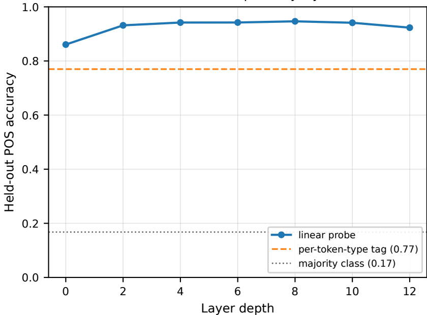
DiffuGPT-S: POS probe by layer
