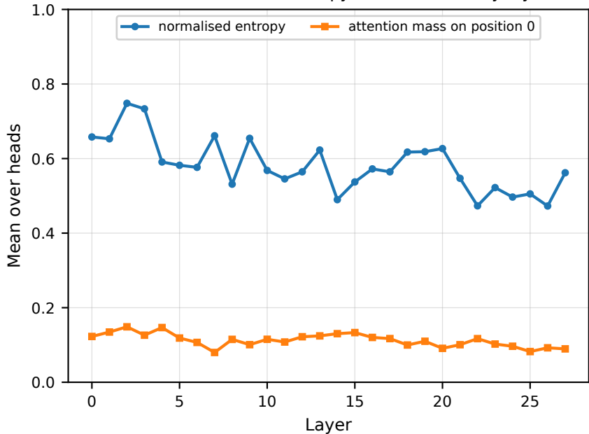
Dream-7B: attention entropy and sink mass by layer
