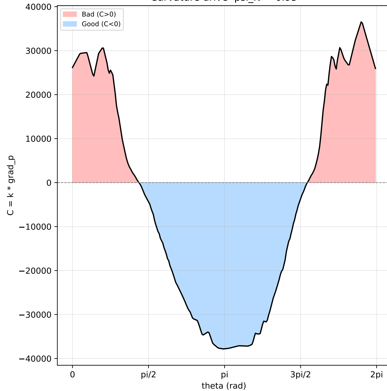
Curvature drive \psi_N = 0.95
