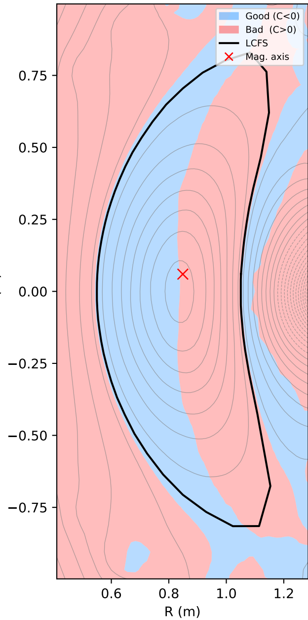
Good / Bad curvature ( C = k \cdot \text{grad}_p )
