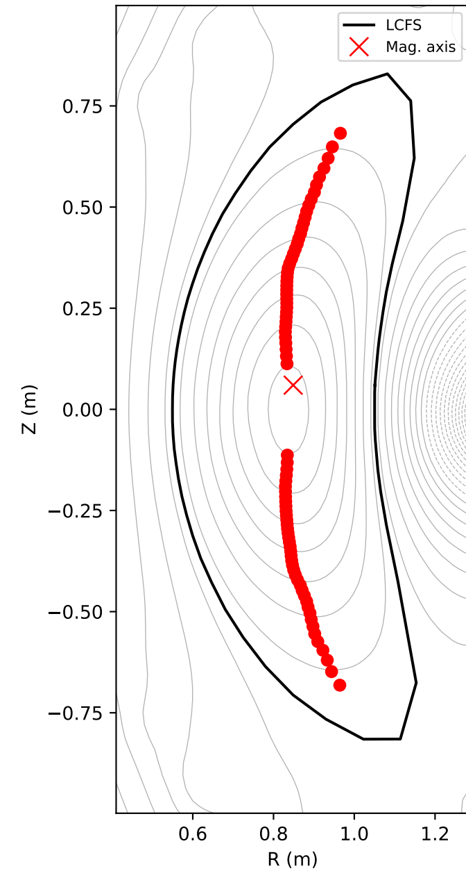
C = 0 loci across flux surfaces
