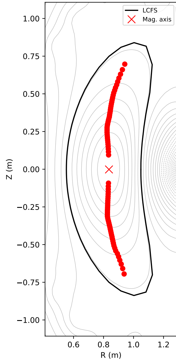
C = 0 loci across flux surfaces
