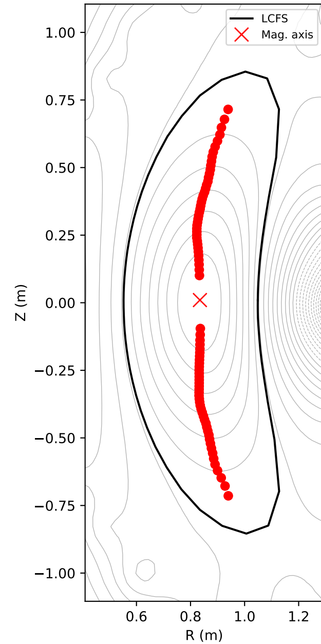
C = 0 loci across flux surfaces
