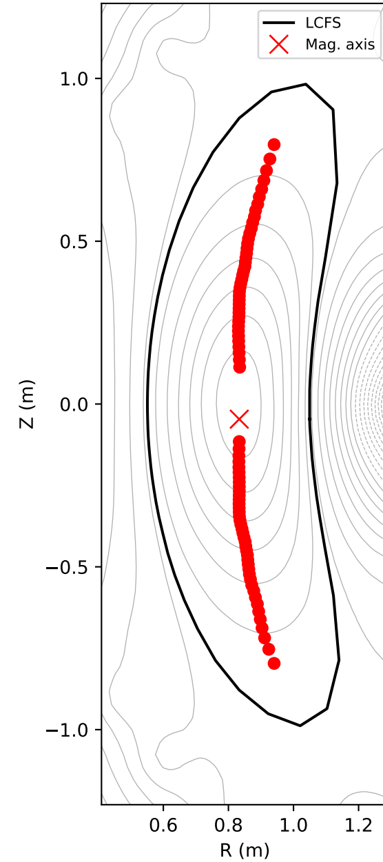
C = 0 loci across flux surfaces
