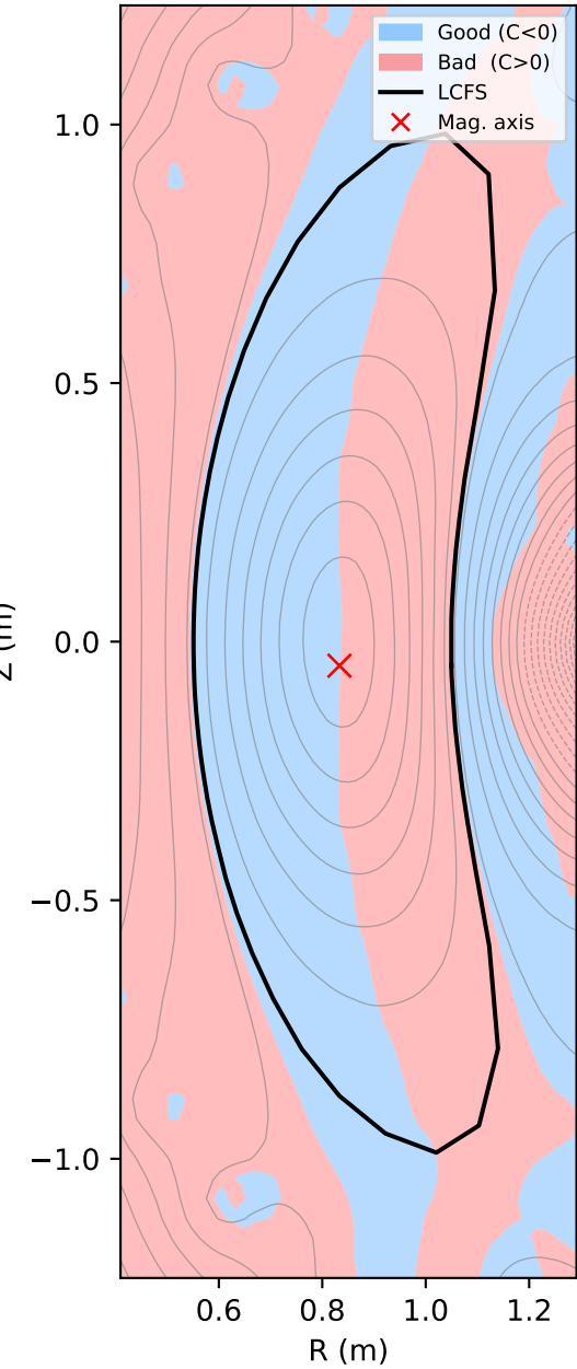
Good / Bad curvature ( C = k \cdot \text{grad}_p )
