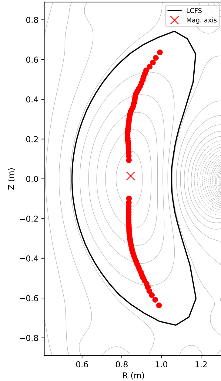
C = 0 loci across flux surfaces
