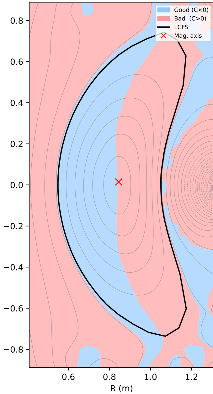
Good / Bad curvature ( C = k \cdot \text{grad}_p )
