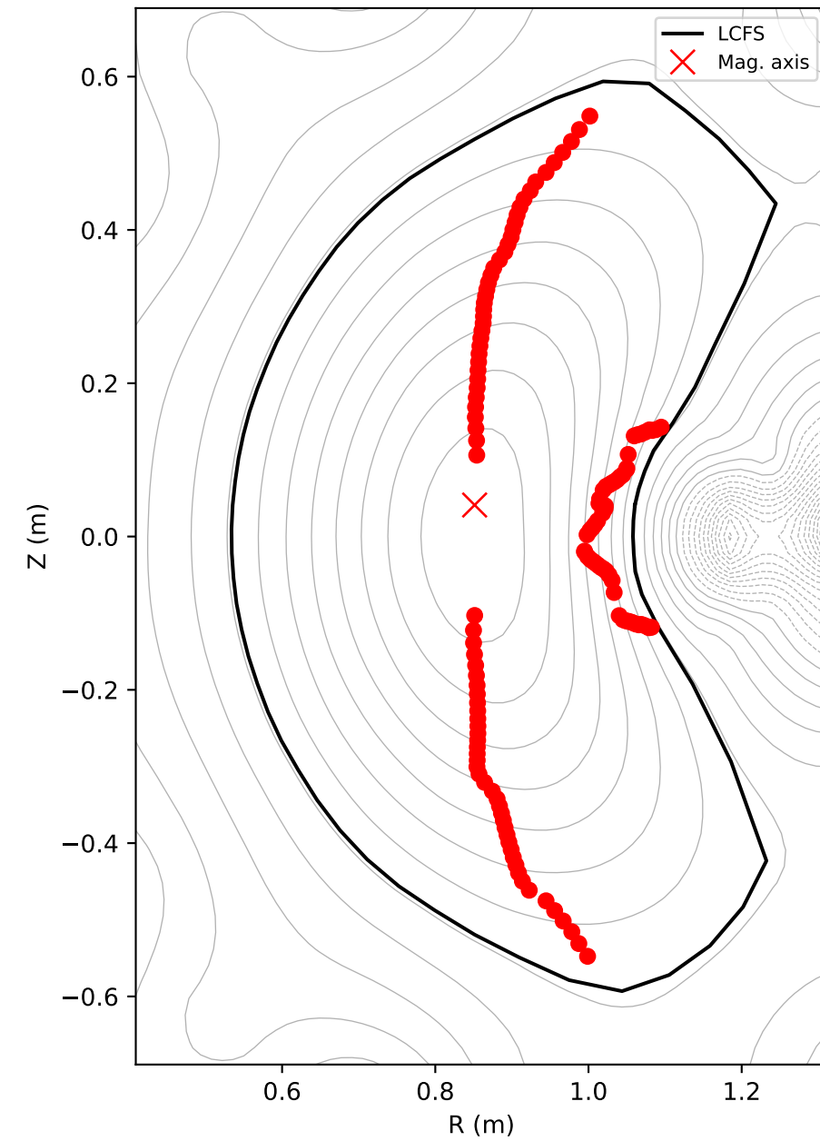
C = 0 loci across flux surfaces
