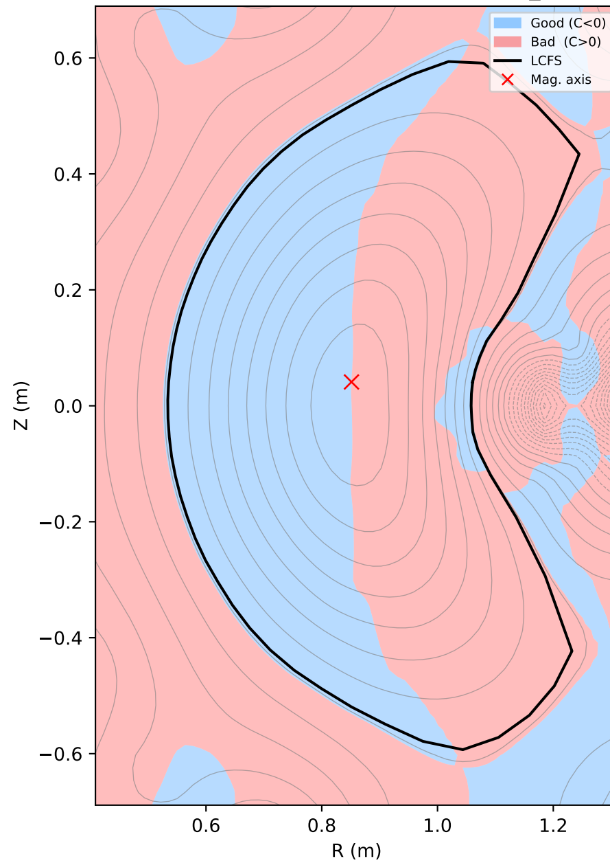
Good / Bad curvature ( C = k \cdot \text{grad}_p )
