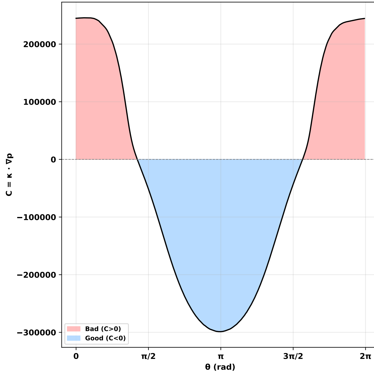
Curvature drive along \psi_N = 0.95
