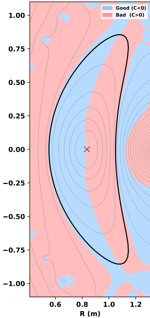
Good / Bad curvature ( C = \kappa \cdot \nabla p )
