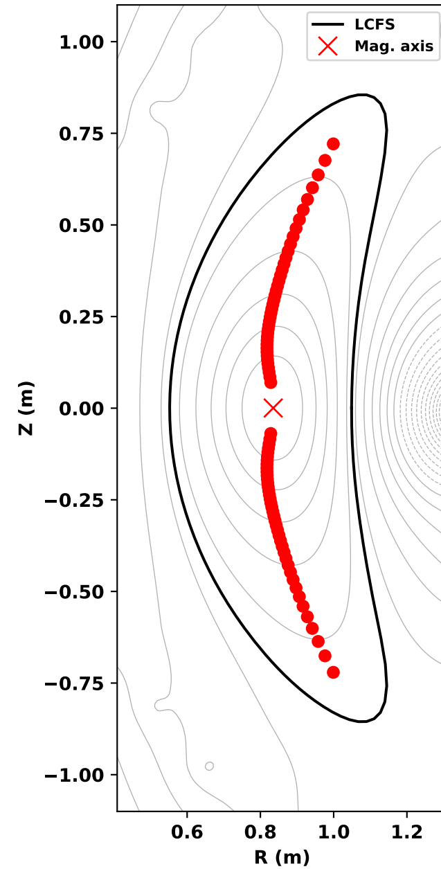
C = 0 loci across flux surfaces
