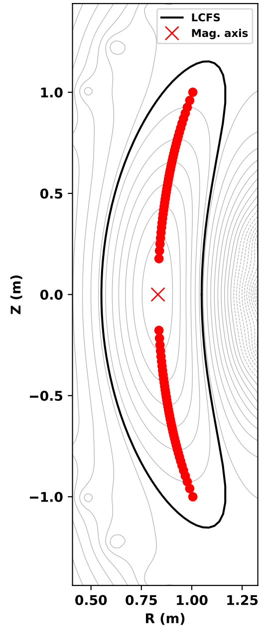
C = 0 loci across flux surfaces
