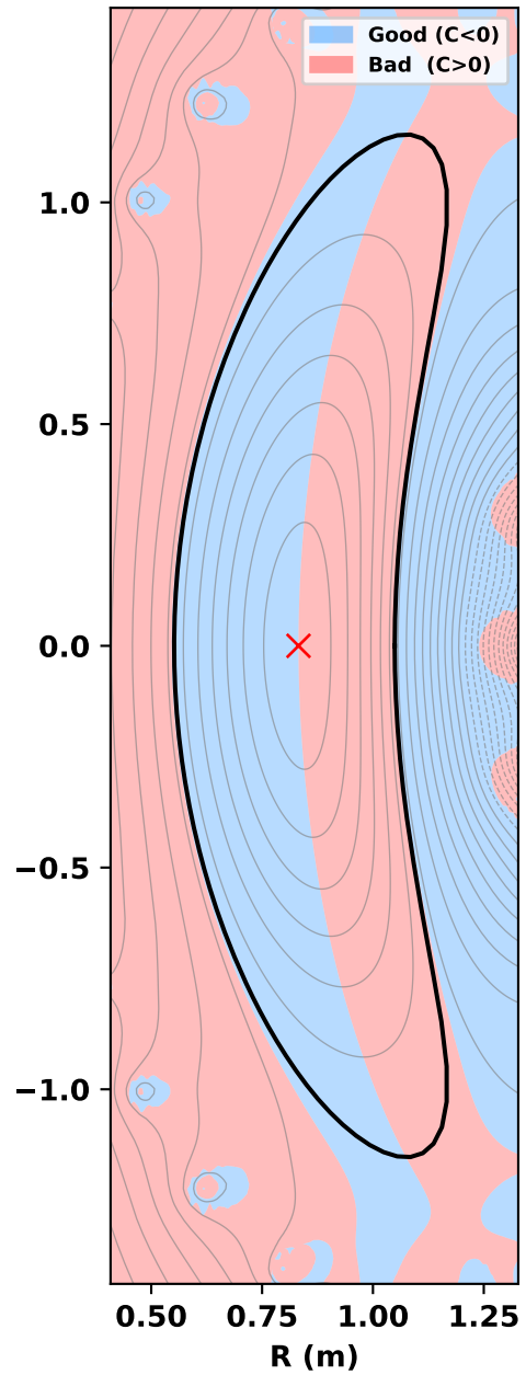
Good / Bad curvature ( C = \kappa \cdot \nabla p )
