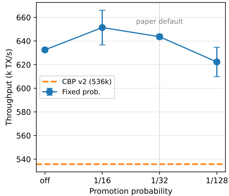
TPC-C
