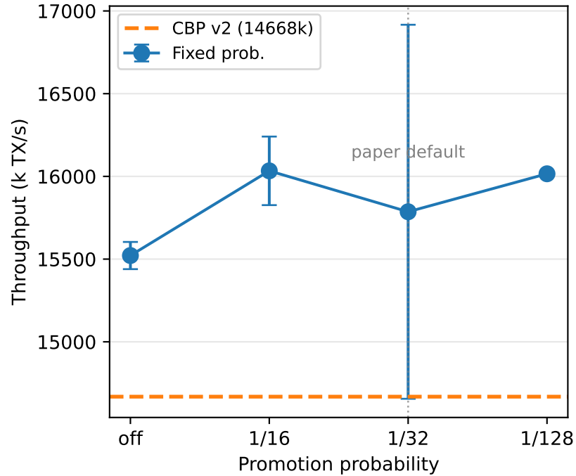
Random Read
