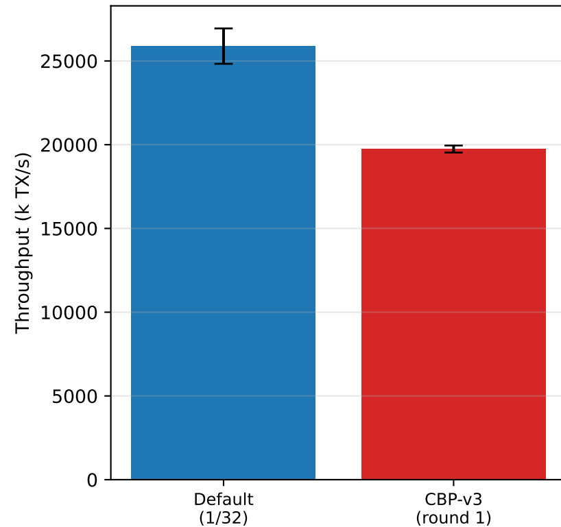
Skewed YCSB
