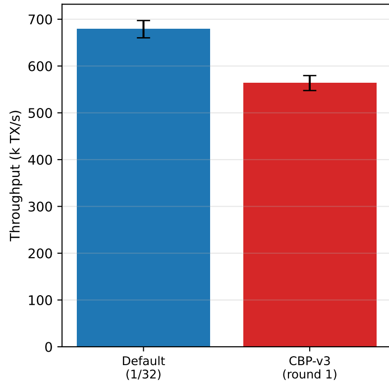
TPC-C
