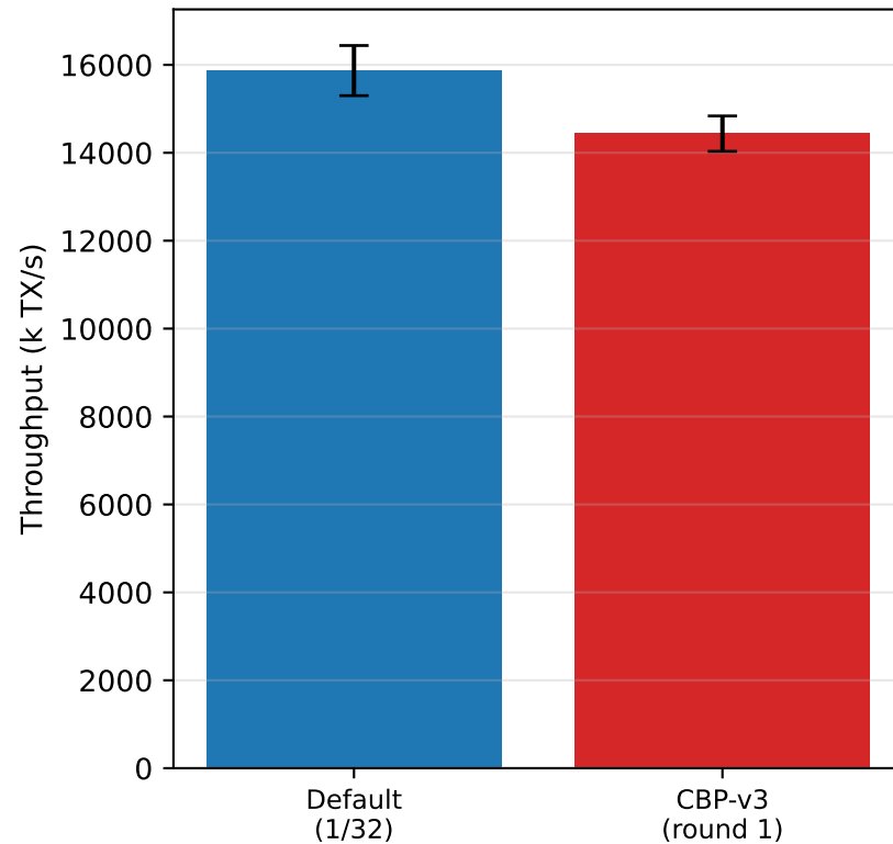
Random Read
