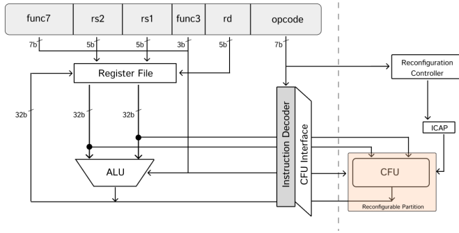
Fig. 2. CFU Playground interface architecture — the standardised handshake between VexRiscv and the Custom Function Unit.
