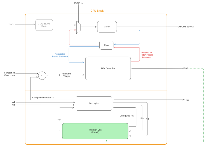
Fig. 1. System block diagram — DFX-integrated CFU Playground architecture showing the static partition, DFX Decoupler boundary, and reconfigurable cfu_compute partition.
