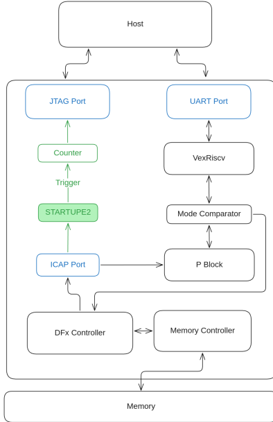
Fig. 5. ICAP-based reconfiguration architecture — the target autonomous path where bitstream storage, retrieval, and delivery occur entirely within the FPGA fabric.
