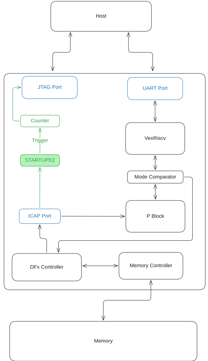
Fig. 5. Fig. 5: ICAP-based reconfiguration architecture — the target autonomous path where bitstream storage, retrieval, and delivery occur entirely within the FPGA fabric.
