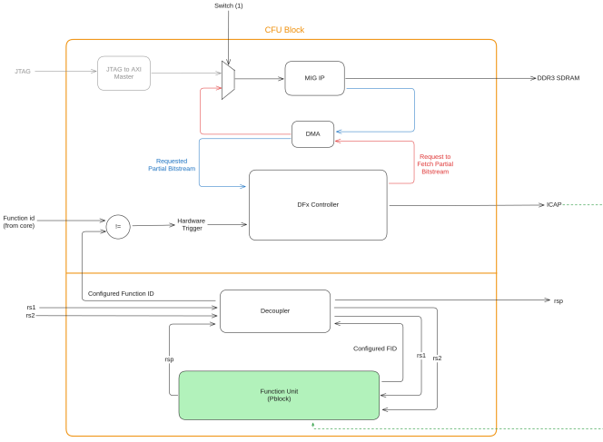
Fig. 1. Fig. 1: System block diagram — DFX-integrated CFU Playground architecture showing the static partition, DFX Decoupler boundary, and reconfigurable cfu_compute partition.
